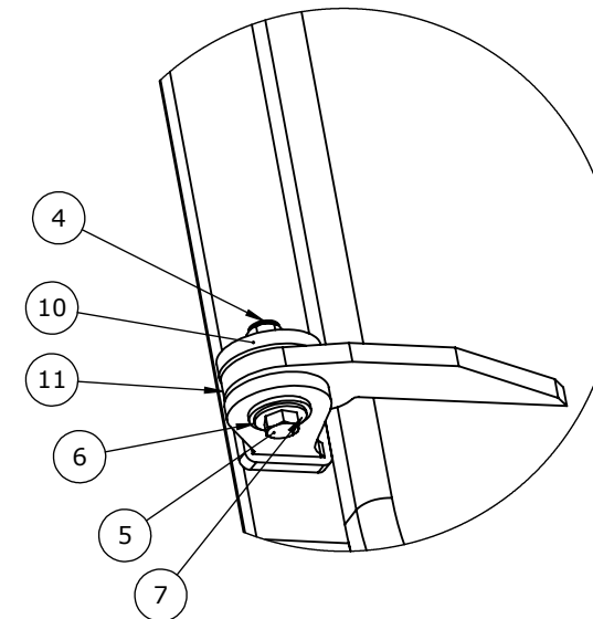
DETAIL J SCALE 1 : 5
