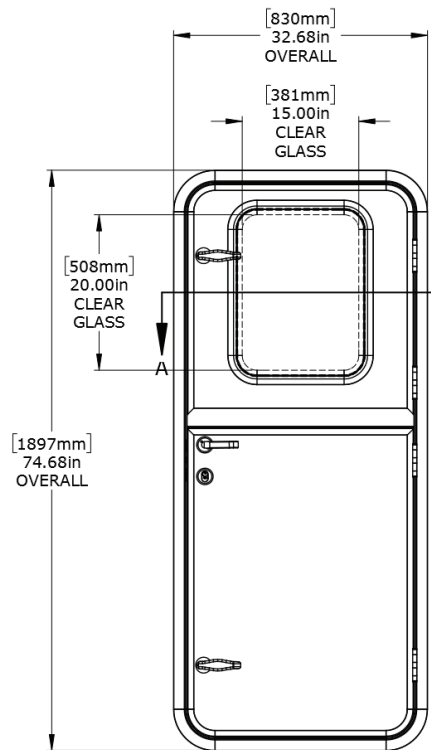
EXTERIOR VIEW
