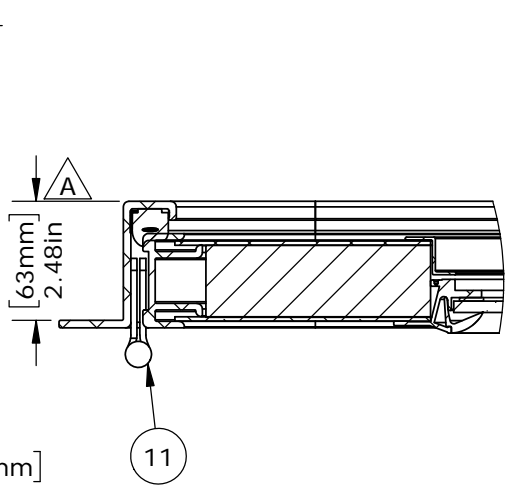
DETAIL B SCALE 1 : 4
