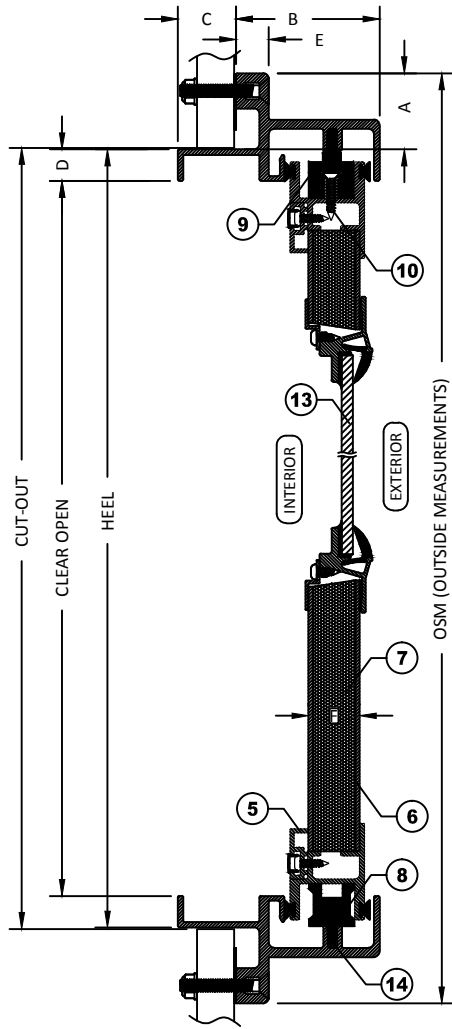
SECTION B-B
