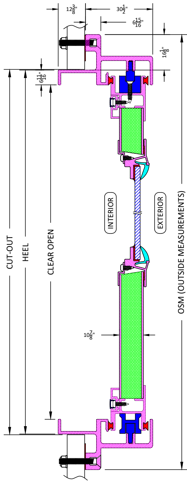
SECTION B-B
