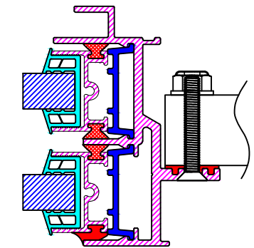
OPTIONAL BOLT-ON INSTALLATION
