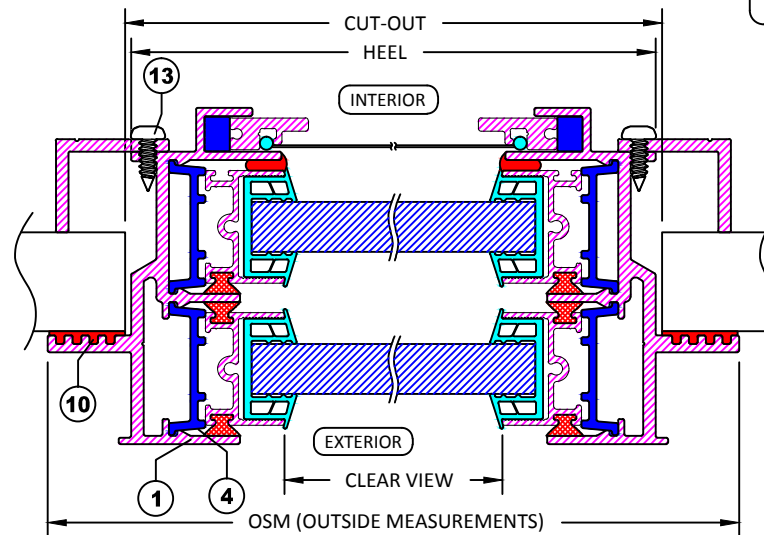
SECTION A-A WITH CLAMP IN INSTALLATION
