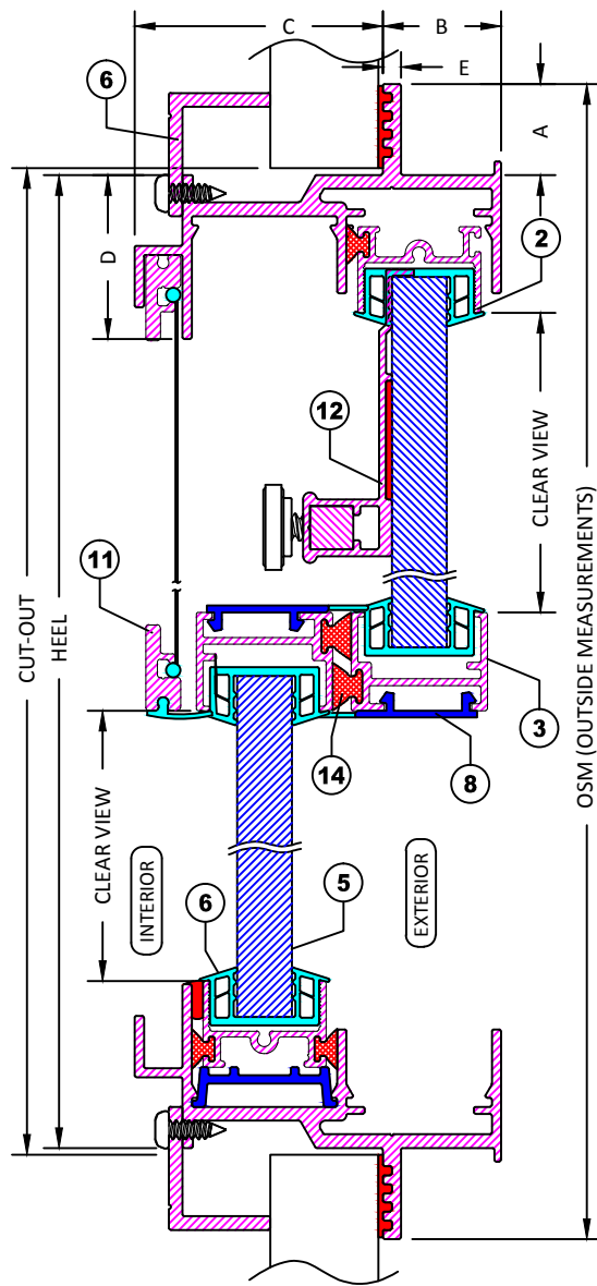
SECTION B-B WITH CLAMP IN INSTALLATION
