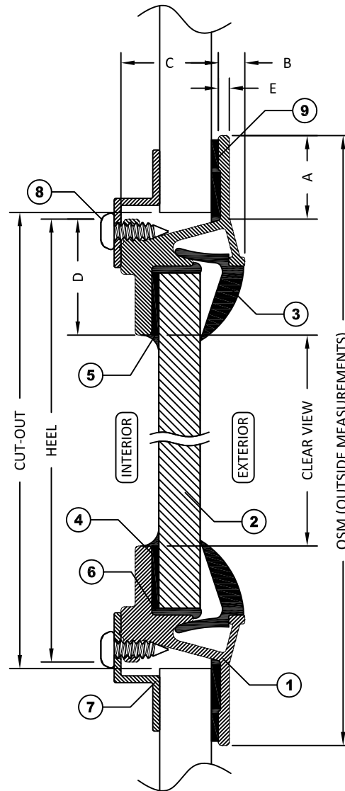
SECTION A-A WITH CLAMP IN INSTALLATION
