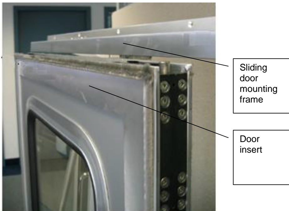
Figure 5 - Sliding door mounting frame
