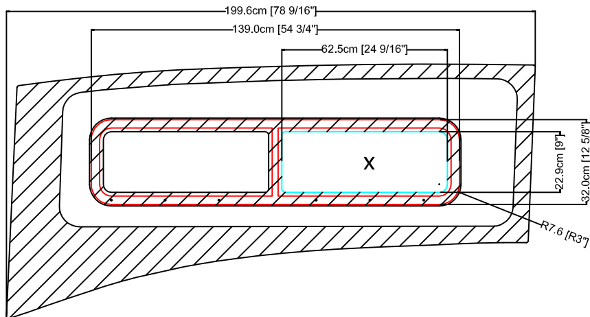
WATERJET STOP (AS VIEWED FROM INSIDE)
