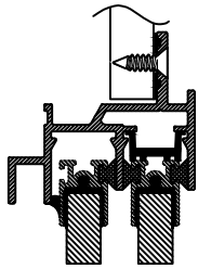
OPTIONAL BOLT-ON INSTALLATION
