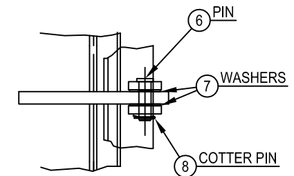
DETAIL OF HINGE
