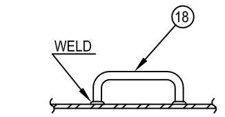
DETAIL OF GRAB HANDLE
