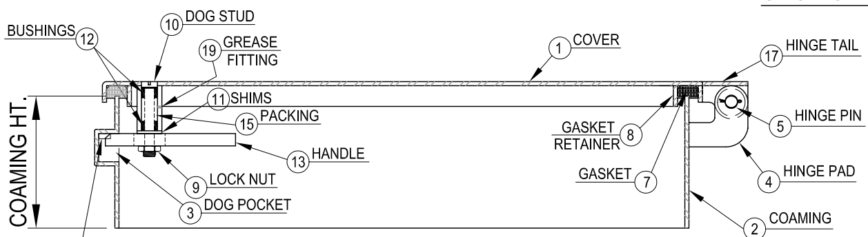
SECTION
