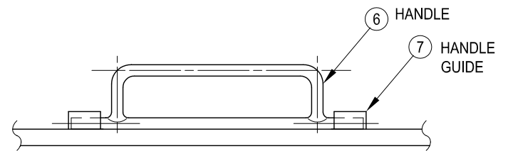
HANDLE DETAIL
