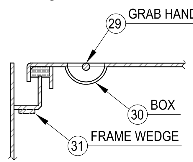
HANDLE DETAIL
