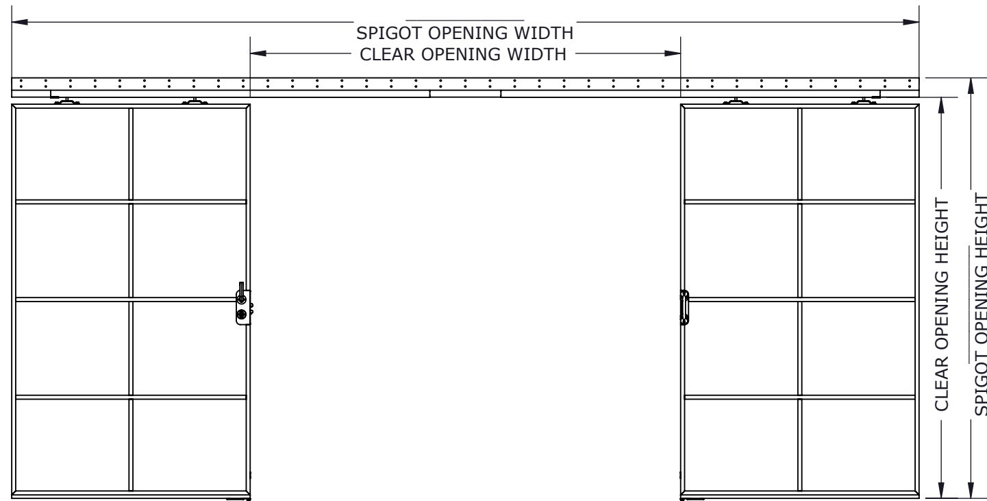
INTERIOR VIEW (OPEN)
